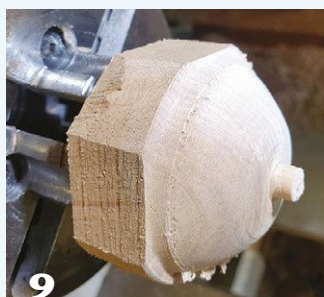
A custom jam chuck is turned from scrap wood, with a \frac{1}{4} " tenon to accept the hole of that size in the bowl. The double-sided tape and the tailstock live center also help hold the bowl in place.
