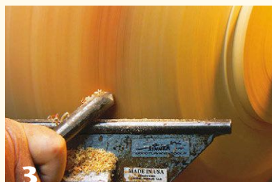
The author remounts a rough-turned, air-dried bowl so it can be trued up using bevel-rubbing and shear-scraping cuts.
