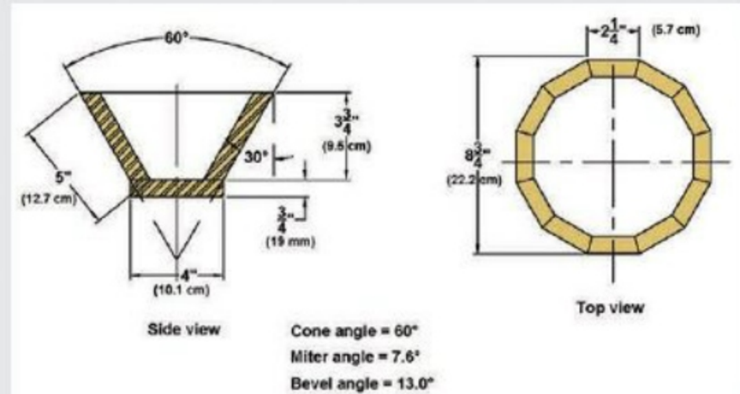
Figure 3. Dimensions and angles for the example project. This is a CAD drawing, but a hand drawing will work just as well.
