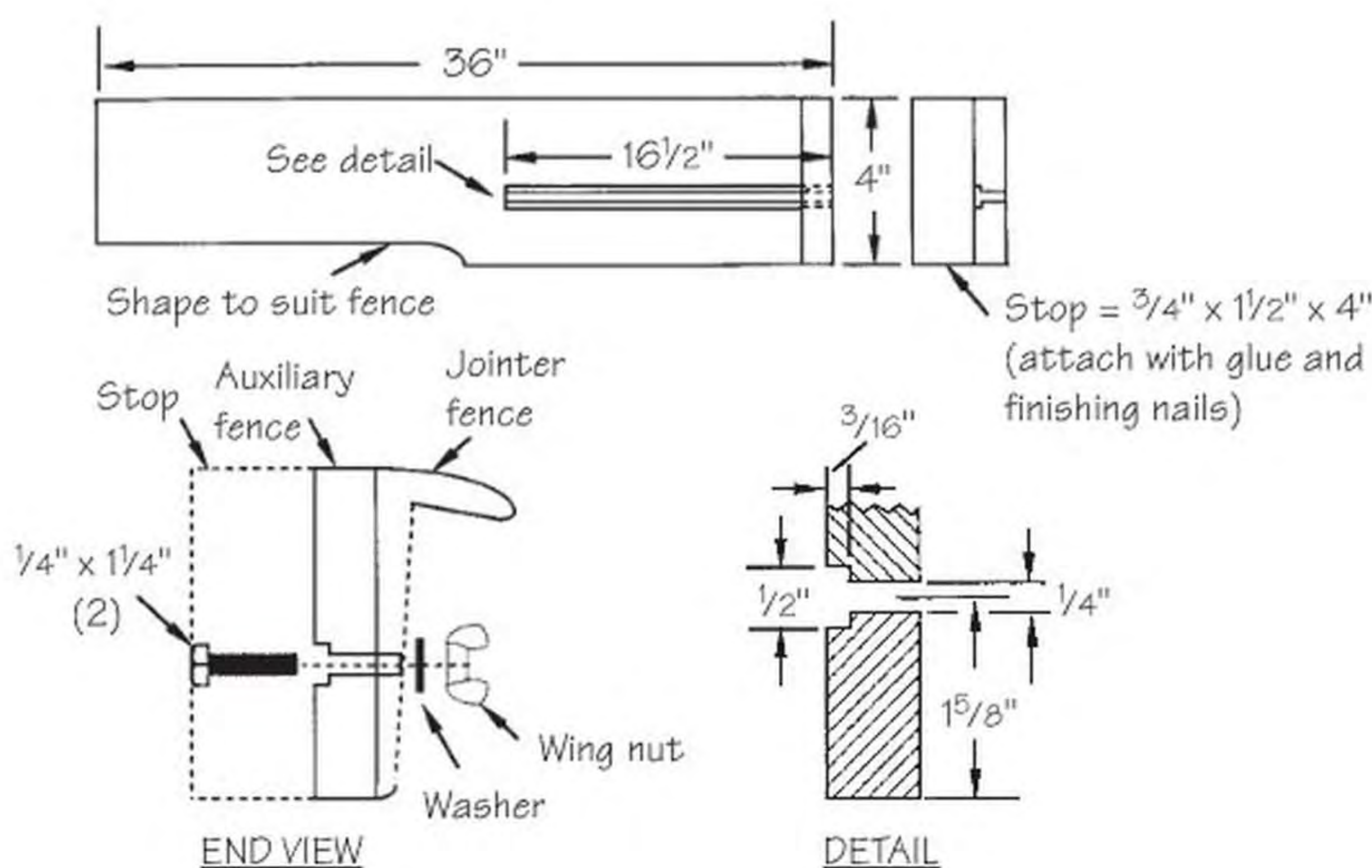
DRAWING 4 AUXILIARY FENCE
