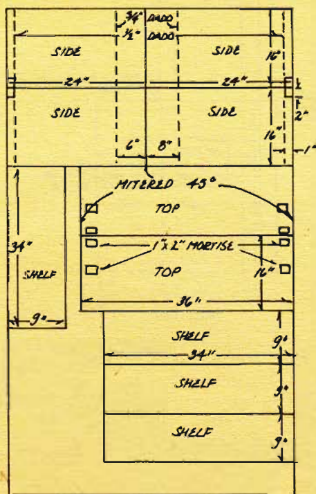
3/4" PLYWOOD FOR TOP, SIDES & SHELVES IN BASE
