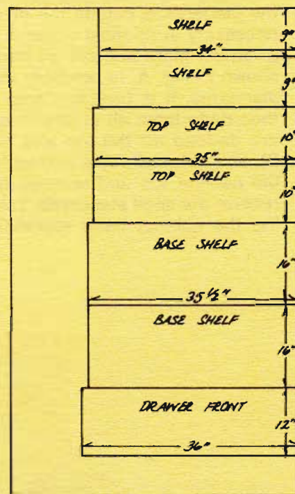
3/4" PLYWOOD FOR SHELVES & DRAWER FRONT
