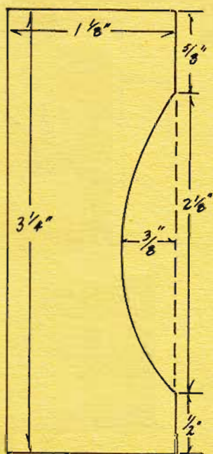
1ST CUT ON TABLE SAW Fig. B
