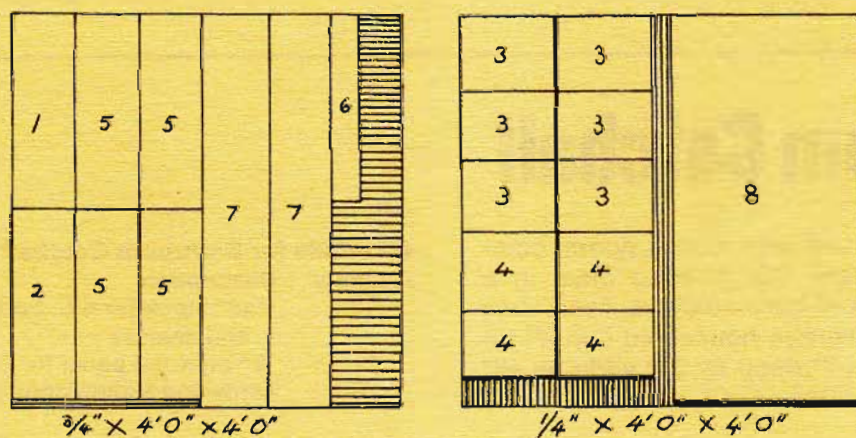
CUTTING DIAGRAM
