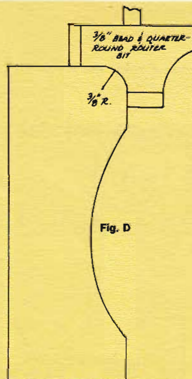
2ND CUT - ROUTER OR BY HAND WITH A BIDGE PLANE
