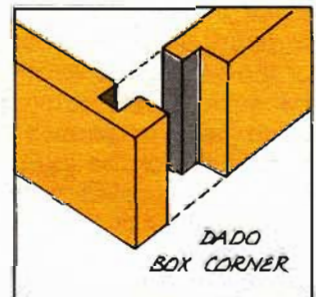
MILLED DADO BOX CORNER
