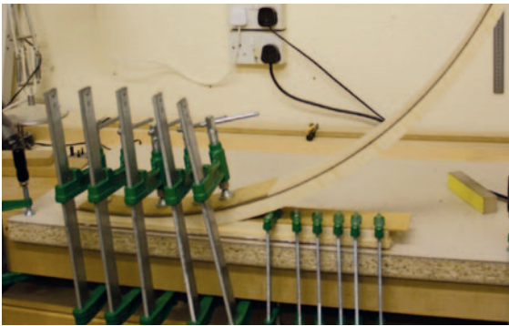
Pic.5 The straight component (C) needs to be rounded at the end to meet the inner (A) curved part of the leg assembly (above, left). These two parts can then be glued and screwed together (above). Once that is done extra laminations are glued to the top of the joint between the straight part (C) and the inner part (A) to cover the joint. The end of the straight part is then mitred (right) to join the outer leg (B)
