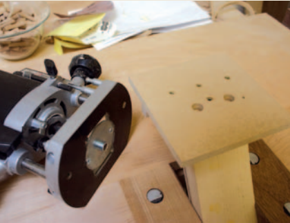
Pic.6 The dowel drilling (or dowel routing) jig is screwed to the mitred end of the straight part of the leg assembly, and then to the mitred end of the outer leg part (B). Steve makes lots of these 'instant' jigs in his work
