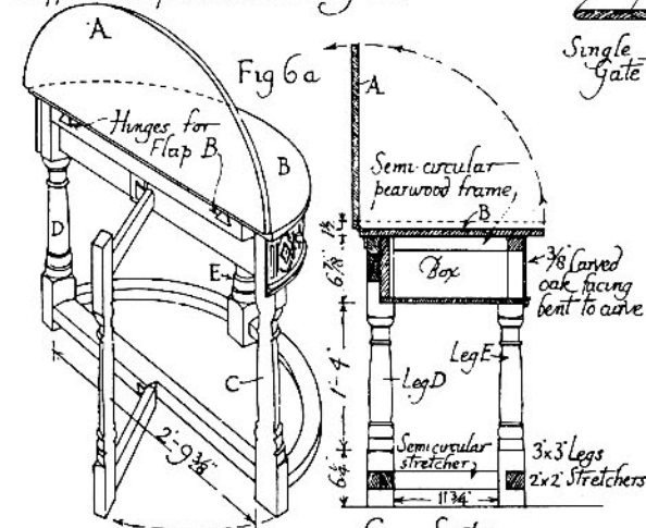
FRAMING DIAGRAM OF THE COMMON GATE LEG TABLE
