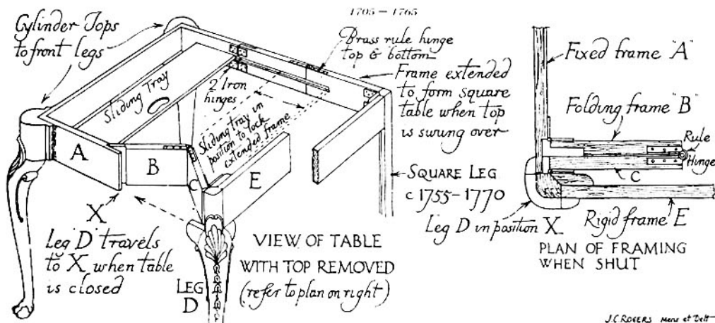
FOLDING FRAME OF CARD TABLES
