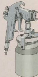
Spray gun and cup Cup serves as finish reservoir; suction feeds finish through metal tube to gun, where compressed air atomizes the liquid into a mist when trigger is pulled
