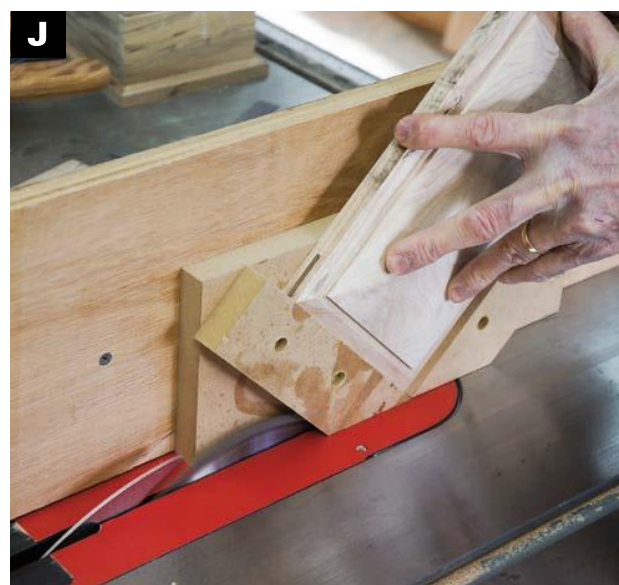
USE A KEYED MITER JIG on the tablesaw to cut grooves in the corners of the lid for miter keys to fit.
