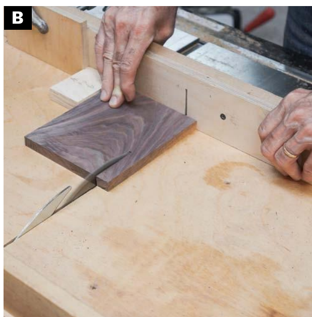
WITH THE SPACER block in place, trim the top panel to the required dimension.
