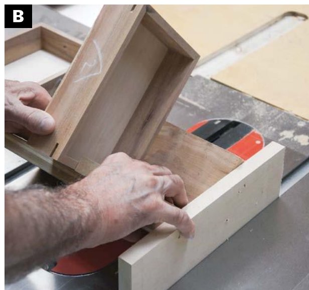
CUT KEYED MITER slots on the tablesaw. A spacer block is used in the keyed miter guide to hold the box in the right position for each cut.
