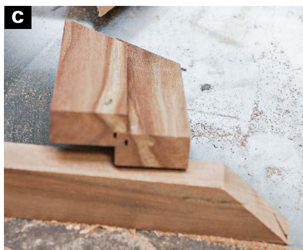
MAKE TEST CUTS to prepare the saw for shaping the top panel and lid sides to fit. A simple interlocking joint as shown is required, both parts made with a single setup of the saw. Set the blade height at \frac{3}{16} in. and the distance between the blade and fence exactly equal to the width of the sawkerf.
