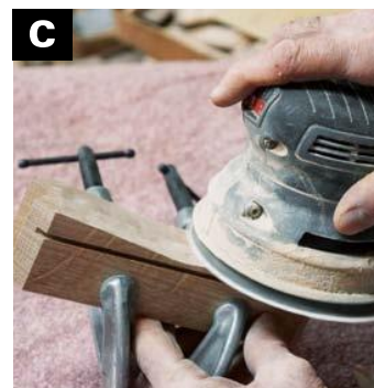
SAND CONCAVE SHAPES using sanding blocks and a random-orbit sander.
