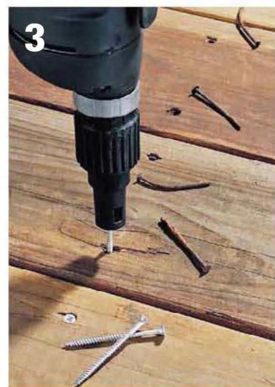
Drive new fasteners to secure loose decking to joists. If using the old nail or screw holes, new fasteners should be slightly longer than the originals.
