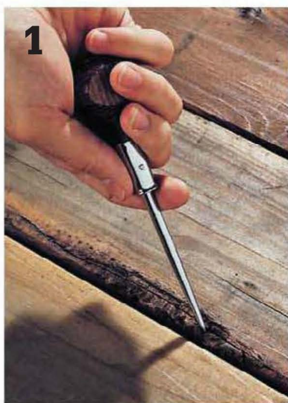
Use an awl or screwdriver to check deck for soft, rotted wood. Replace or reinforce damaged wood.
