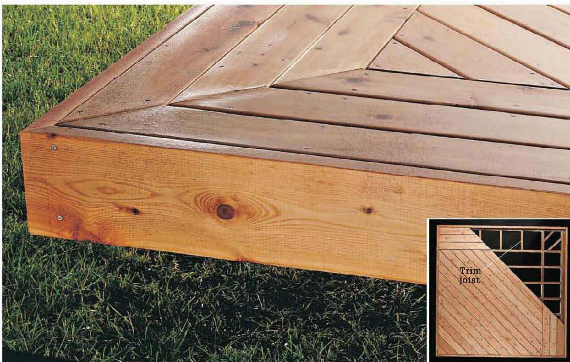
Border pattern gives an elegant, finished look to a deck. Install trim joists to support the border decking.
