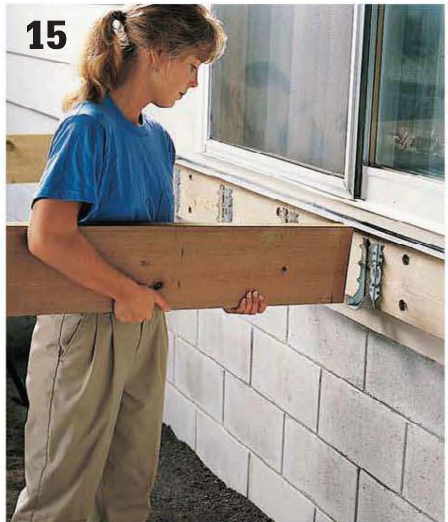
15 Seal cut ends with clear sealer-preservative. Place joists in hangers with crowned edge up.
