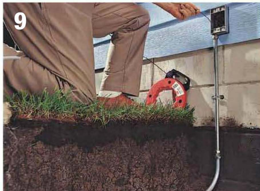
At the house, use fish tape to pull cable through the conduit and into the GFCI box.
