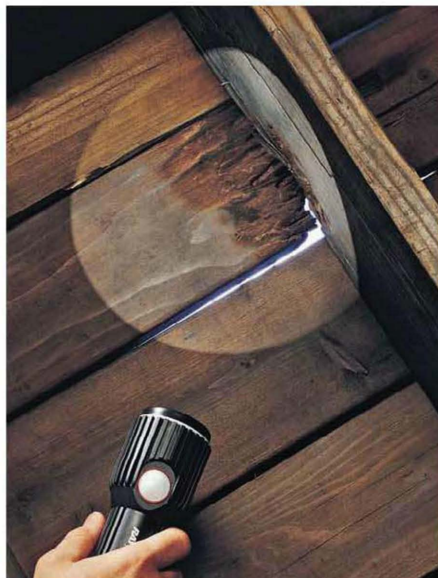
Inspect hidden areas regularly for signs of rotted or damaged wood. Apply a fresh coat of finish yearly.
