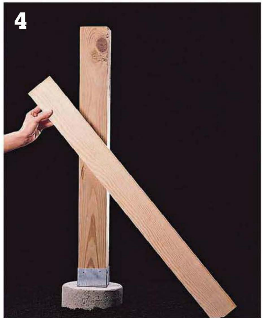
4 Brace post with a 1 x 4. Place the 1 x 4 flat across post so that it crosses the post at a 45° angle about halfway up.
