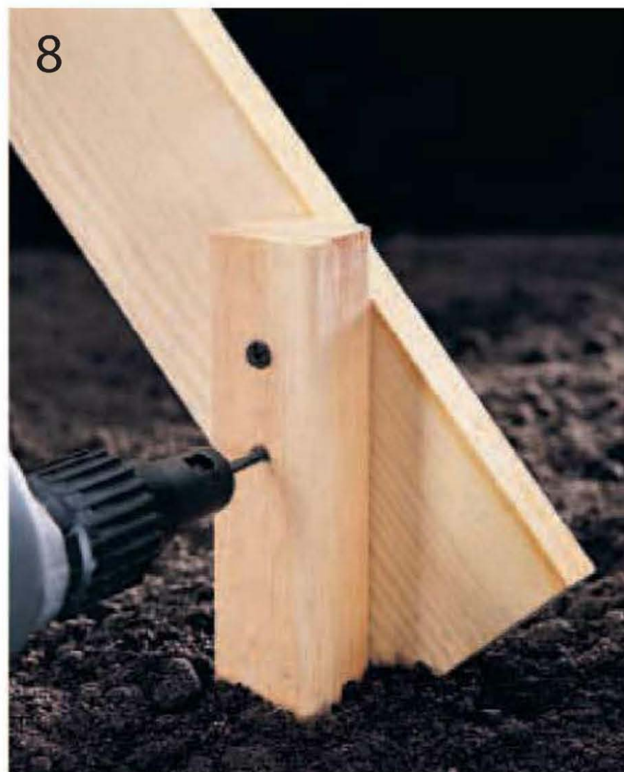
8 Attach the brace to the stake with two 2" wallboard screws.
