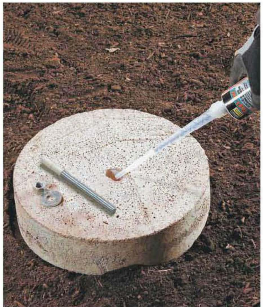
High strength epoxy and threaded rod are good options for attaching metal connecting hardware to concrete footings.
