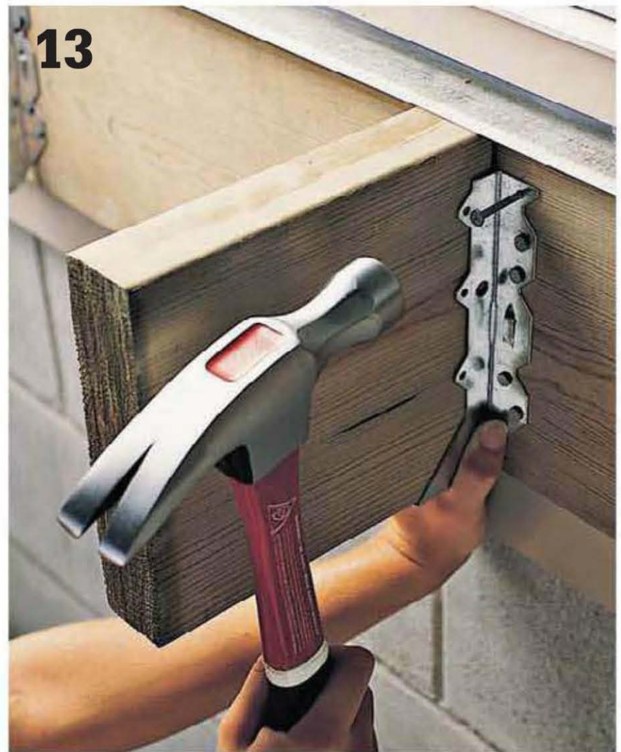
13 Nail the remaining side flange to the framing member with 10d joist hanger nails. Remove spacer.
