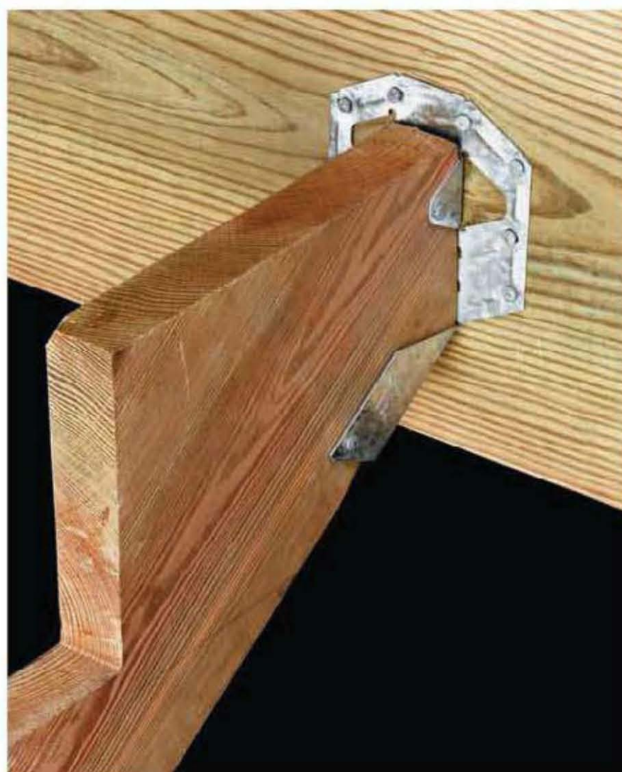
Skewable joist hangers attach 2x lumber, such as stair stringers, to the face of framing at an adjustable angle.
