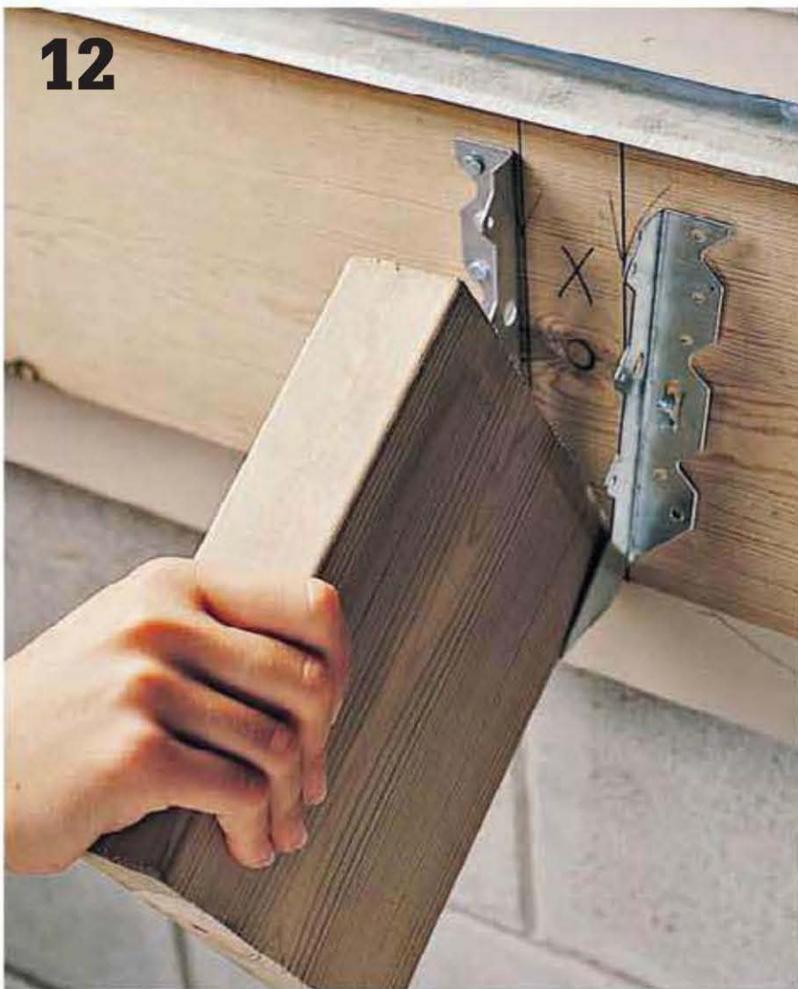
12 Cut a scrap board to use as a spacer. Hold spacer inside each joist hanger, then close the hanger around the spacer.
