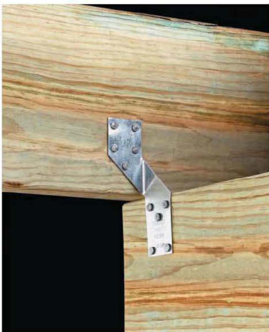
Seismic ties attach 2x joists or rafters to the top of a beam at its ends.
