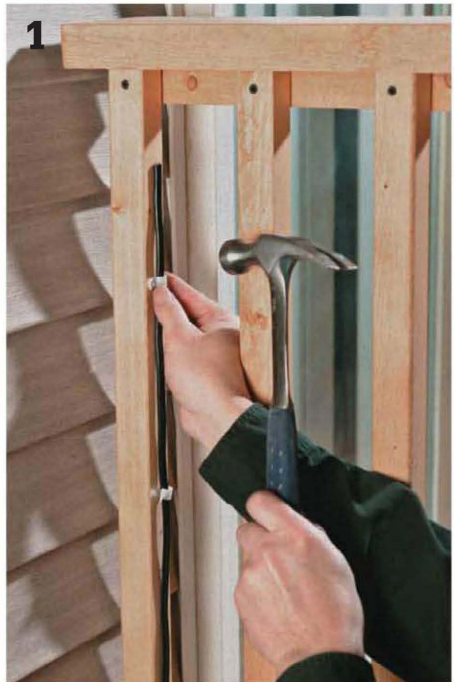
Run low-voltage cable from a transformer or low-voltage circuit to the end of the railing and secure with cable staples.
