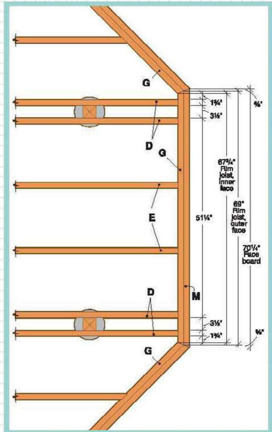
Detail B
