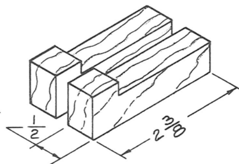
Illus. 2-41. The guide block with the hole drilled.
