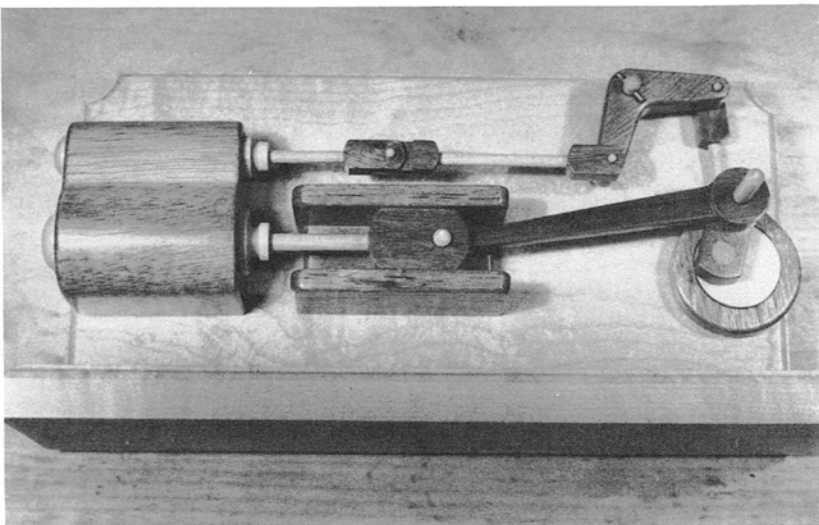
Illus. 3-74. Final assembly: Step three.
