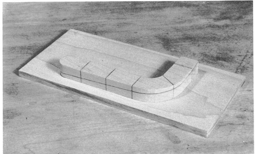
Illus. 4-13. The insert glued to the baseplate.
