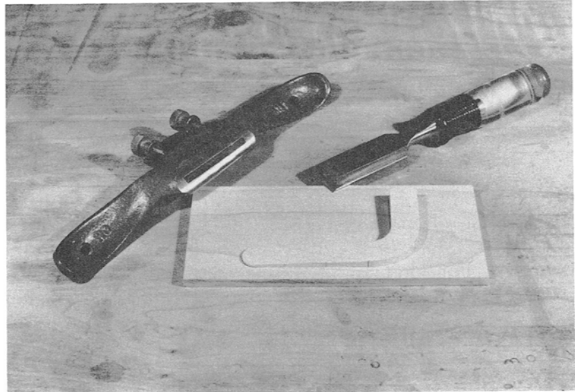
Illus. 4-14. You can remove most of the stock with a chisel and trim to the line with a spokeshave.
