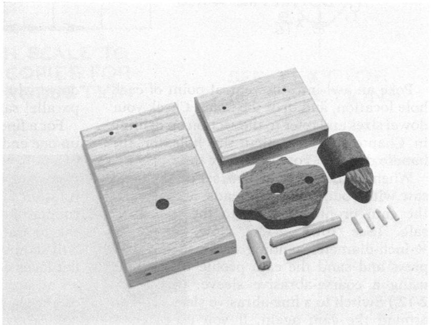
Illus. 2-7. All the parts for the Cam and Follower mechanism.
