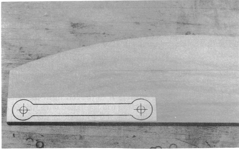
Illus. 4-28. The connecting-rod pattern glued to the wood.
