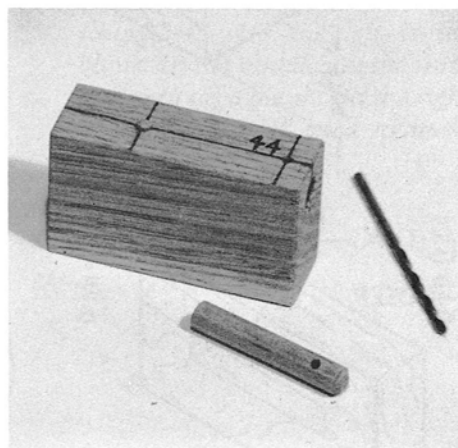
Illus. 2-39. This drill jig is used to drill a pin hole for a \frac{1}{4} -inch-diameter axle.
