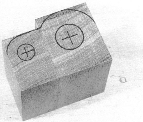
Illus. 3-18. The cylinder block laid out.
